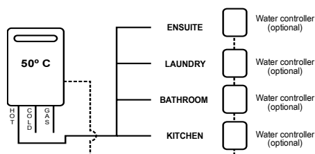
Diagram 1 - 50°C Appliance
