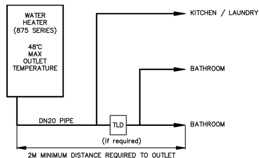
875 Series - No Controllers
