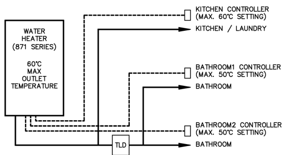
Note: NZ - max Kitchen Controller and outlet temperature is 55°C 871 Series - Kitchen and Bathroom Controllers
