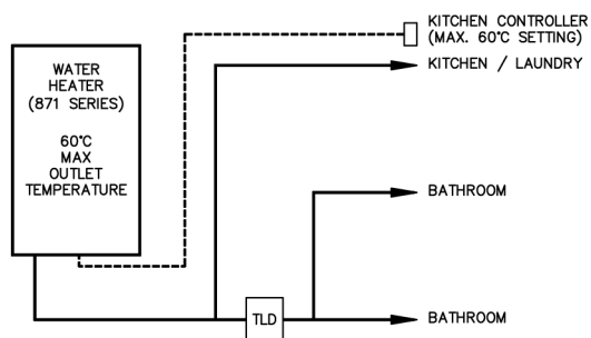
Note: NZ - max Kitchen Controller and outlet temperature is 55°C 871 Series - Kitchen Controller Only
