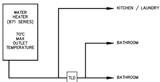
Note: NZ - maximum outlet temperature is 75°C 871 Series - No Controllers
