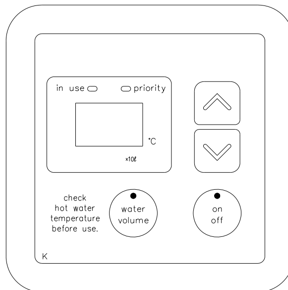
Kitchen Controller
